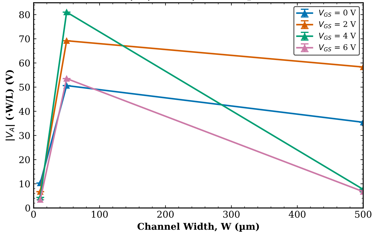
TFT2 Transistor 1 |V_A| vs W | L = 40\text{ }\mu\text{m}
